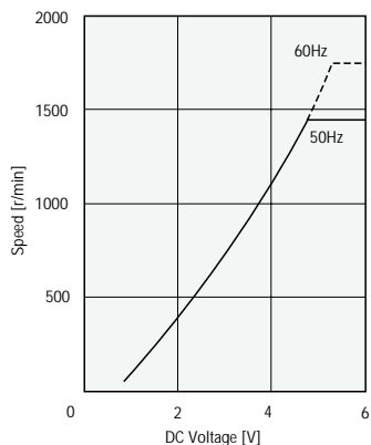
Speed Setting Voltage-Speed Characteristics
