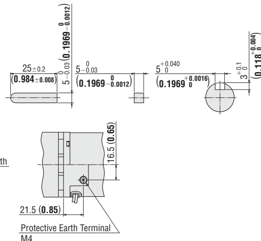
Detail Drawing of Protective Earth Terminal
