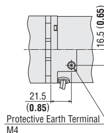
Detail Drawing of Protective Earth Terminal
