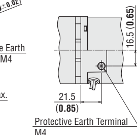
Detail Drawing of Protective Earth Terminal
