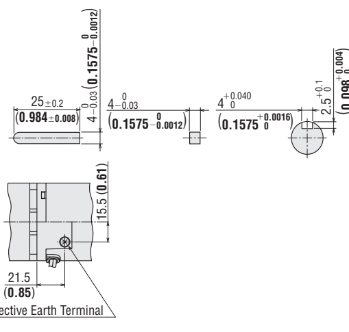
Detail Drawing of Protective Earth Terminal
