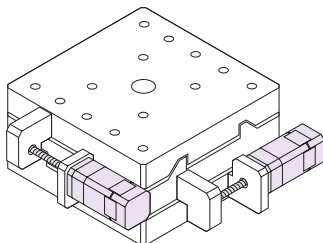
Driving an X-Y Stage (Automated micrometer head)
