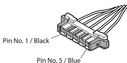
Connection cables
